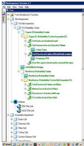
Authoring Tree
